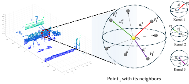
Figure 3. A point i within a point cloud, along with its 7 neighboring points and 3 kernels. Unlike other graph methods, this approach uses direction to obtain structural information.
